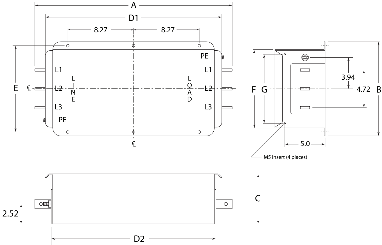
Typical Dimensions:
